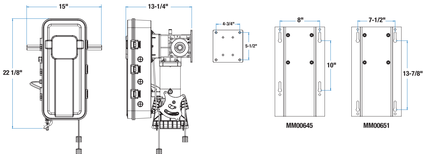
MV00541 Electromechanical Brake Kit
