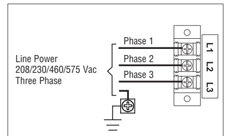
Three Phase Power Wiring
