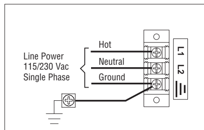
Single Phase Power Wiring
